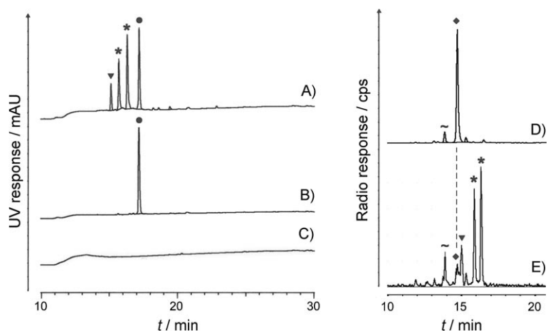
Figure 1. LCMS chromatograms; A = crude crDA reaction of 12 and 6 after four days: ( \blacktriangledown ) = isomer B (10.1%), (*) = isomer A 1 (21.3%), (*) = isomer A 2 (33.2%), and ( \bullet ) = residual c (RGD) 12 (34.2%). B = c (RGD) 12 . C = oxanor-DTPA derivative 6 . Radiolabel traces; D = ( \blacklozenge ) ^{111}\text{In} -oxanor-DTPA complex ( 7 ). E = reaction mixture comprised of ( \blacktriangledown ) = byproduct in starting material ( \blacklozenge ) = ^{111}\text{In} -DTPA-labeled \text{CF}_3 -furan formed concomitantly with product B , (*) = isomer A 1 , (*) = isomer A 2 .
