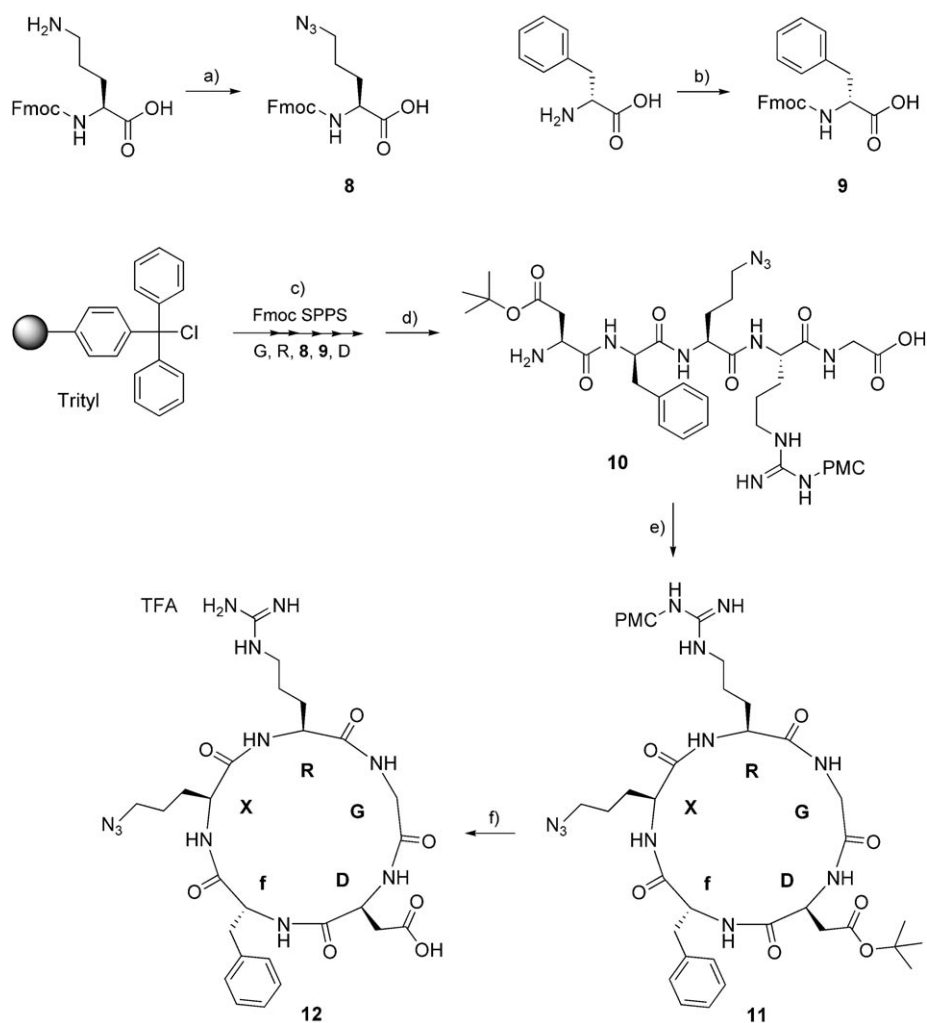
Scheme 2. a) \text{TfN}_3 , \text{CuSO}_4 \cdot \text{H}_2\text{O} (64%); b) FmocCl, DiPEA, 1,4-dioxane (91%); c) Fmoc-based SPPS; d) TFA, TIPS, \text{H}_2\text{O} (90:4.75:4.75) (29% over two steps); e) DPPA, \text{NaHCO}_3 , DMF (87%); f) TFA, \text{CH}_2\text{Cl}_2 (93%).
