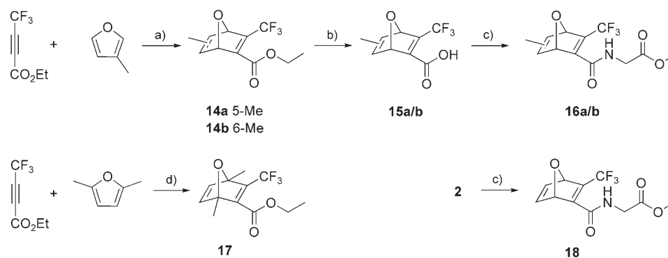
Scheme 5. a) Neat, 40 °C ( 14a/b 72%); b) THF, 1 M NaOH, ( 15a/b 80%); c) H-Gly-OMe, DMAP, EDC, CH 2 Cl 2 (74% for 16a/b ; 56% for 18 ); d) 1,4-dioxane, reflux (91%).
