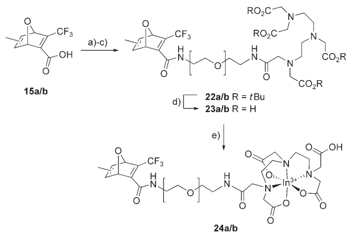
Scheme 7. a) N -Boc-3,6-dioxo-octane-1,8-diamine, EDC, DMAP, CH 2 Cl 2 (47% for 20a/b ); b) TFA, CH 2 Cl 2 (99% for 21a/b ); c) tetra- O - tert -Bu-DTPA, EDC, DMAP, CH 2 Cl 2 (44% for 22a/b ); d) TFA, CH 2 Cl 2 (99%); e) NH 4 OAc buffer (pH 5.5), InCl 3 .
