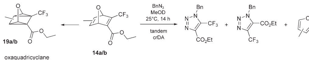
Scheme 6. Formation of oxa-quadracyclanes 19a/b from compound 14a/b upon submission to tandem crDA reaction conditions.
