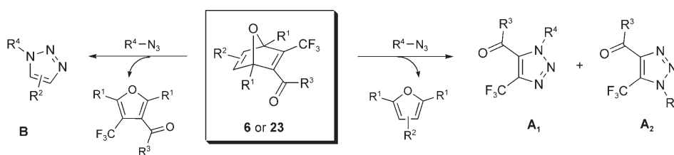
Scheme 4. Reaction pathways for the formation of triazole compounds A 1 , A 2 , and B in the tandem crDA reaction.
