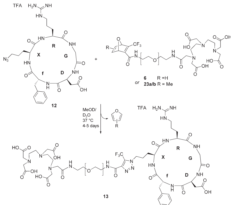
Scheme 3. Conjugation experiment of N - \delta -azido-cyclo-(Arg-Gly-Asp-D-Phe-Orn) 12 with oxanor-DTPA ( 6 ) or Me-oxanor-DTPA ( 23 ) resulting in c (RGD)-CF 3 -triazole-DTPA conjugate 13 (major 1,4-isomer shown).
